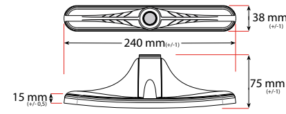
NERI INDUSTRIAL LINE Art. 3006
