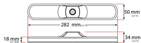
NERI INDUSTRIAL LINE Art. 2002
